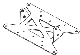
(1)Monitor Bracket-a
